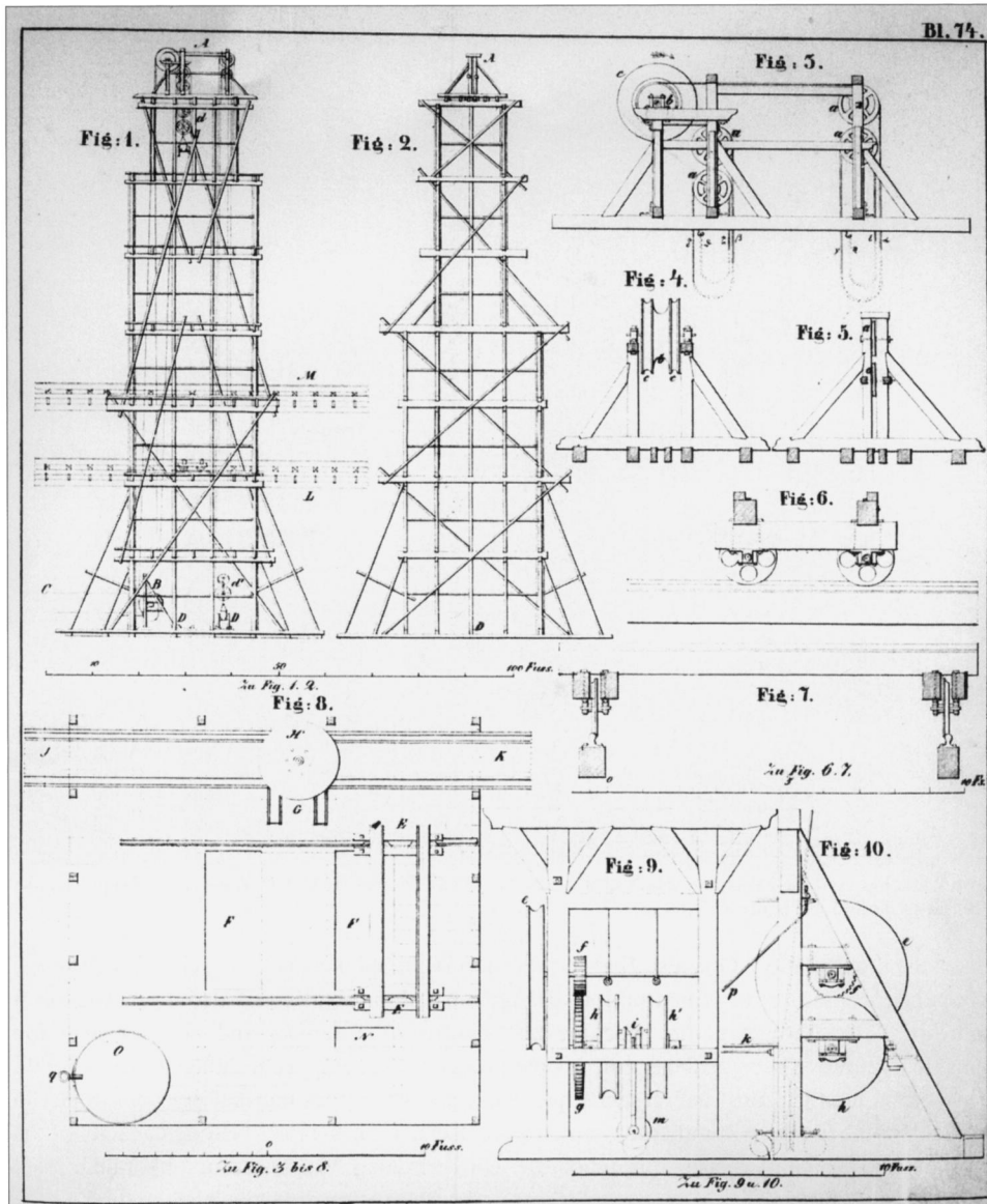
Fig. 8 Neues Museum, wooden hoist in the centre of the future museum with trucks for supplying materials (from Notizblatt des Architektenvereins zu Berlin , 1842).
