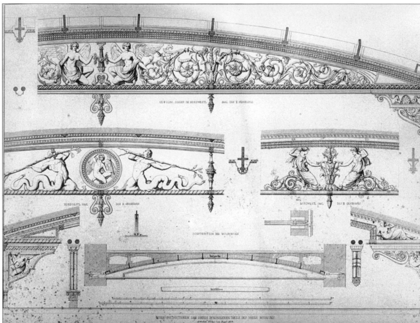
Fig. 16 Neues Museum, bowstring girders, details of iron structure and zinc decoration, published by the architect (from A. Stüler, Das Neue Museum in Berlin , 1862).
