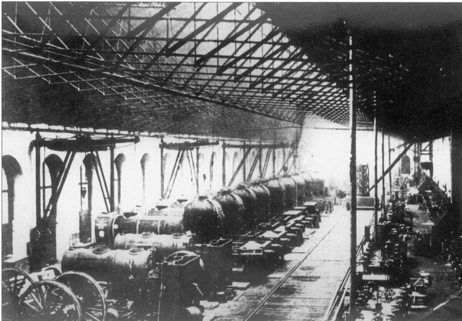
Fig. 5 Borsig's factory at the Chausseestrasse, locomotive assembly room (photograph of 1856 from D. Vorsteher, Borsig, 1983).
