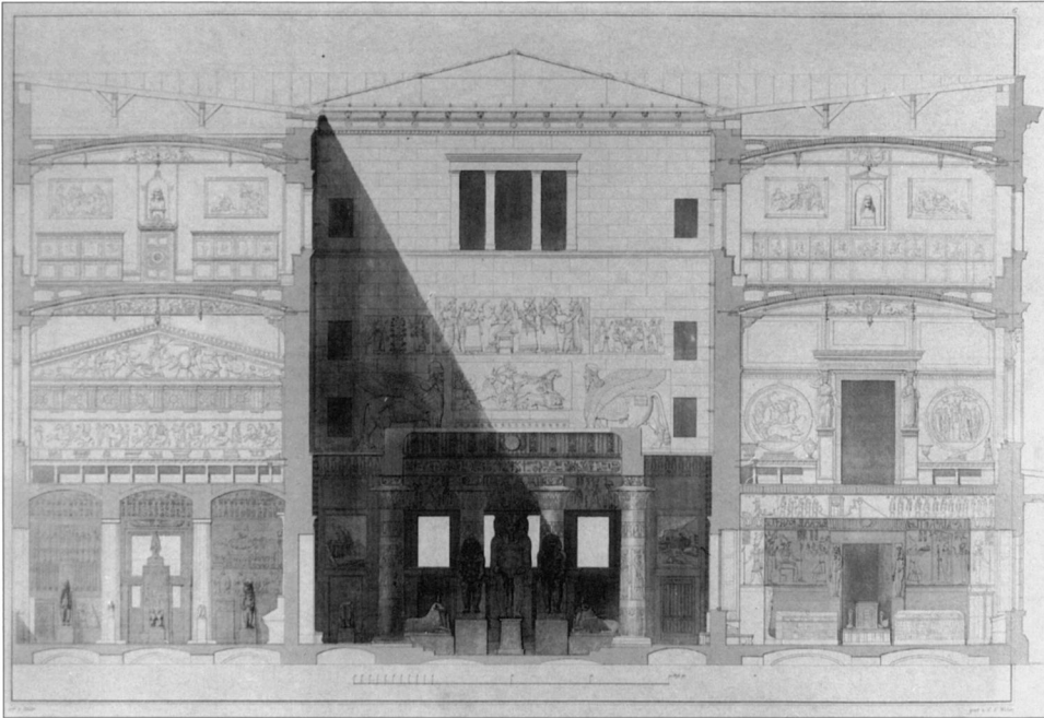
Fig. 15 Neues Museum, northern wing, cross section with bowstring girders, published by the architect (from A. Stüler, Das Neue Museum in Berlin , 1862).
